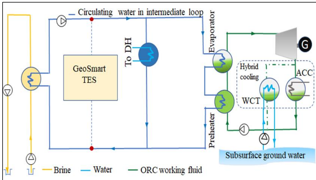
Figure 2. Description of proposed system (Balmatt)
