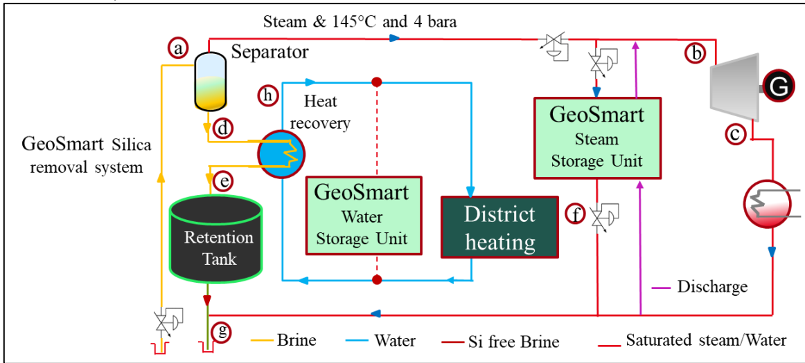
Figure 1. Description of proposed system (Zorlu)
